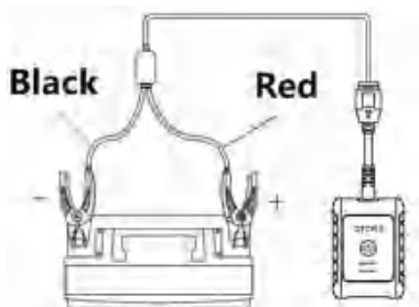
Figure 6-2 Connecting to a Battery
