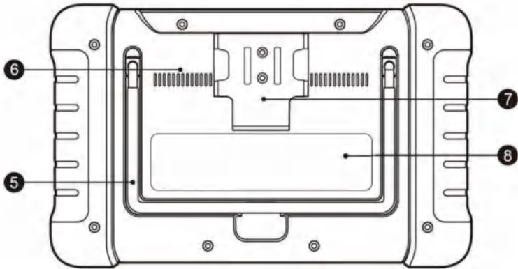
Figure 2-2 Display Tablet Back View
