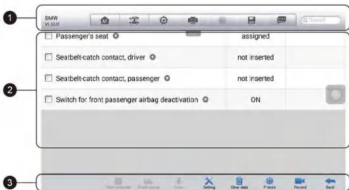
Figure 4-13 Sample Live Data Screen
