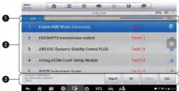
Figure 4-9 Sample Auto Scan Operation Screen
